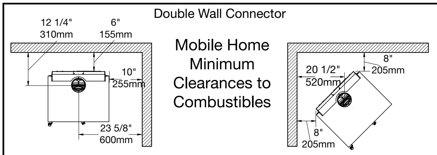
Figure 19: NEOVUE 2.5 mobile home clearances.
