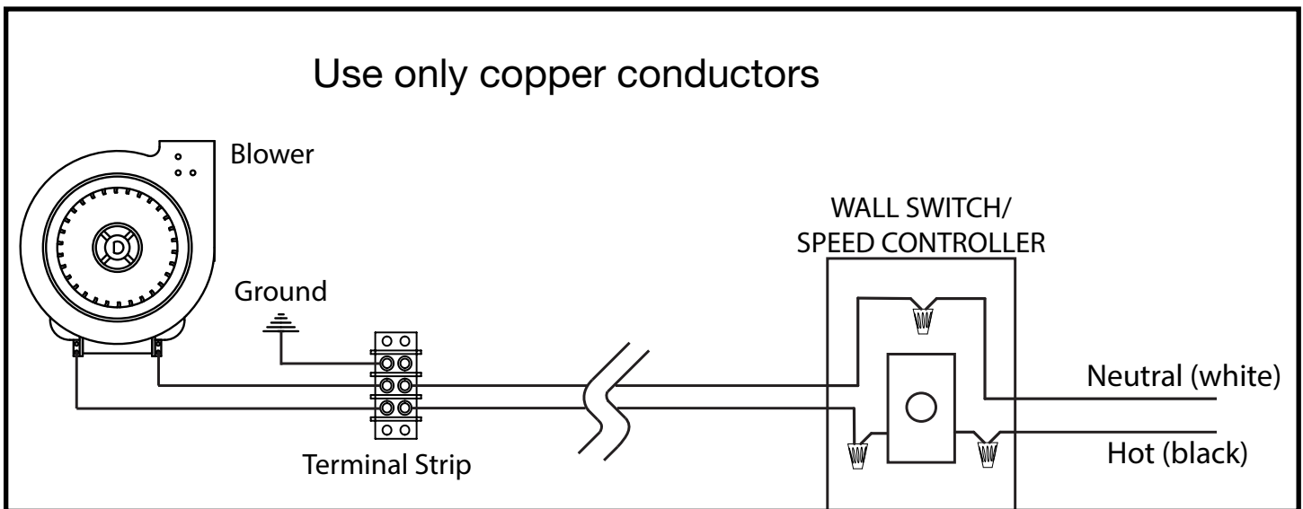
Figure 28: Remote heat kit wiring diagram.
