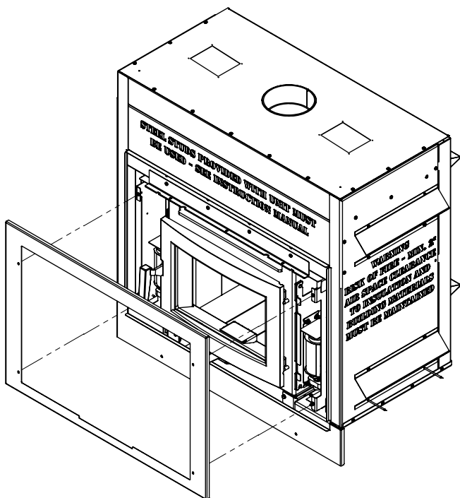
Figure 30: FP25 LE Backing Plate.
