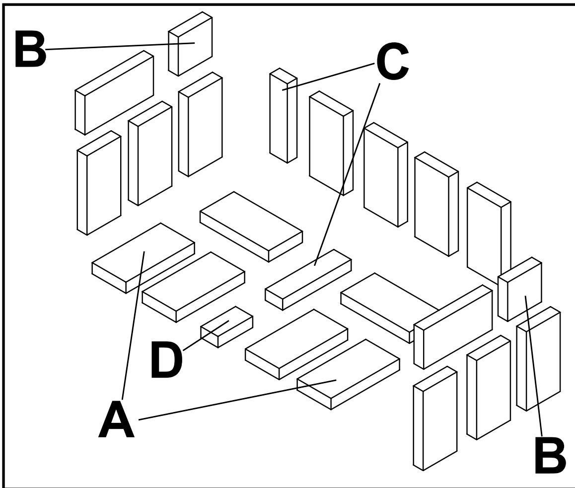
Figure 34: FP25LE Firebrick layout.
