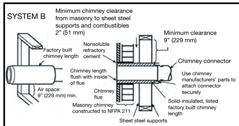
Figure 12: System B Minimum Clearance 9 in. (229mm) to combustibles
