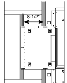
8.5" from stud center to stud center
