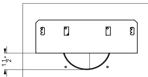
Set 3 (Vent restrictor at 1.5")
