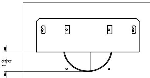
Set 2 (Vent restrictor at 1.75")
