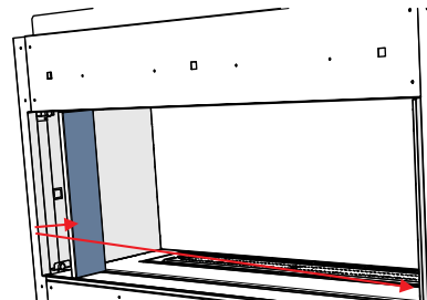
Outer side panel install
