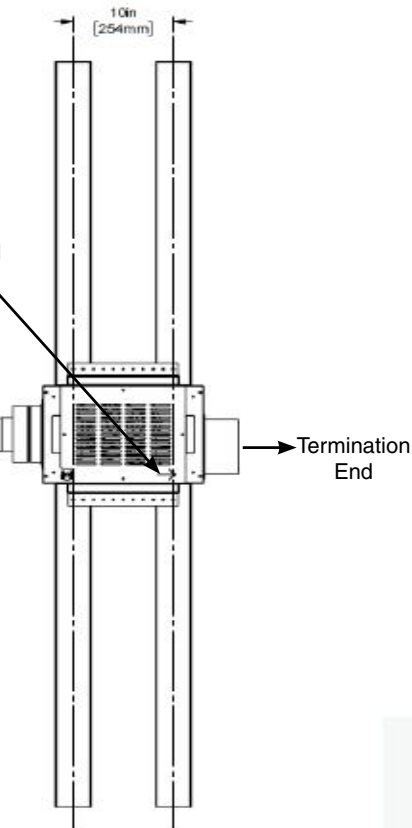
Diagram 2: Inline power vent oriented horizontally
