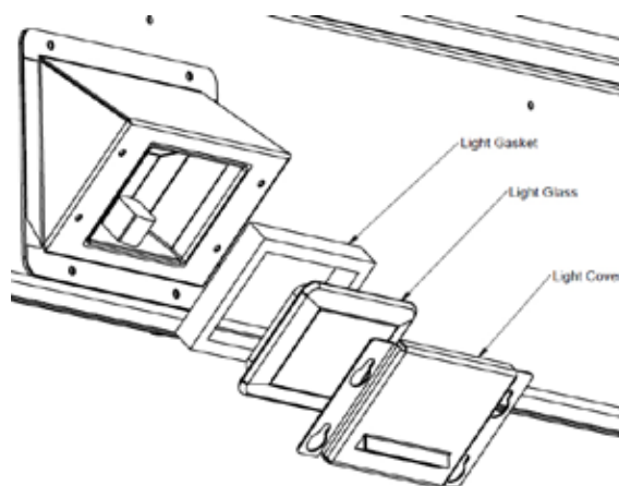
Inner light cover reassembly order
