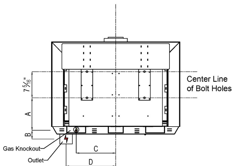
Back View
