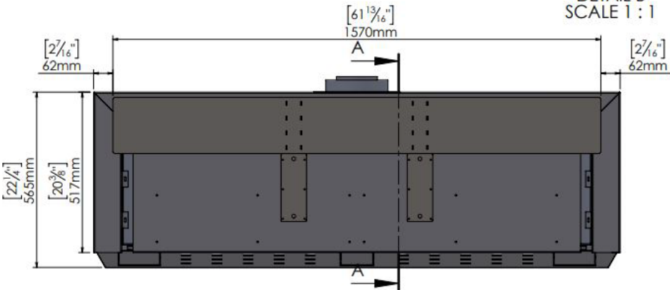
DETAIL B SCALE 1 : 1
