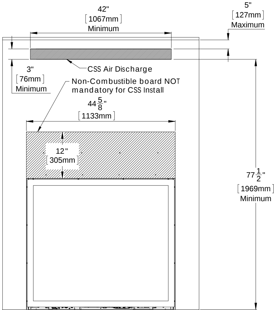
Figure 39: Framing Option 1
