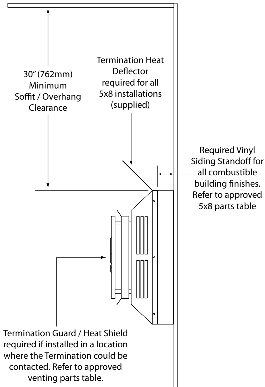
Figure 60: Additional Termination Restrictions for 5" x 8" Venting
