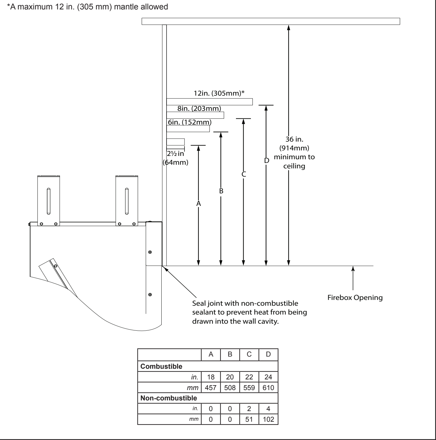
Figure 7.2 Minimum Vertical and Maximum Horizontal Mantel Dimensions For Combustible and Non-combustible Materials
