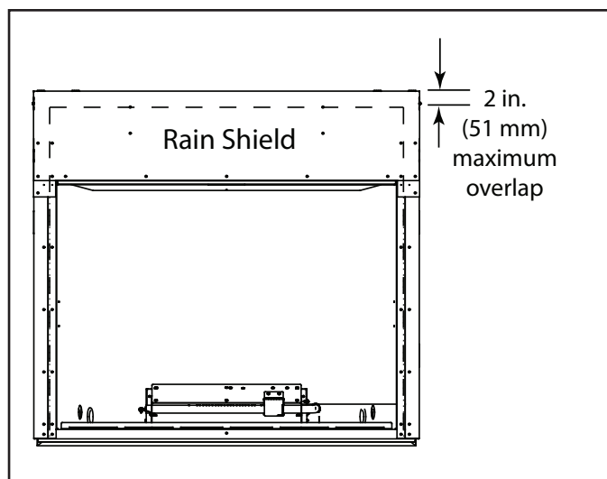
Figure 3.11 Membrane Overlap
