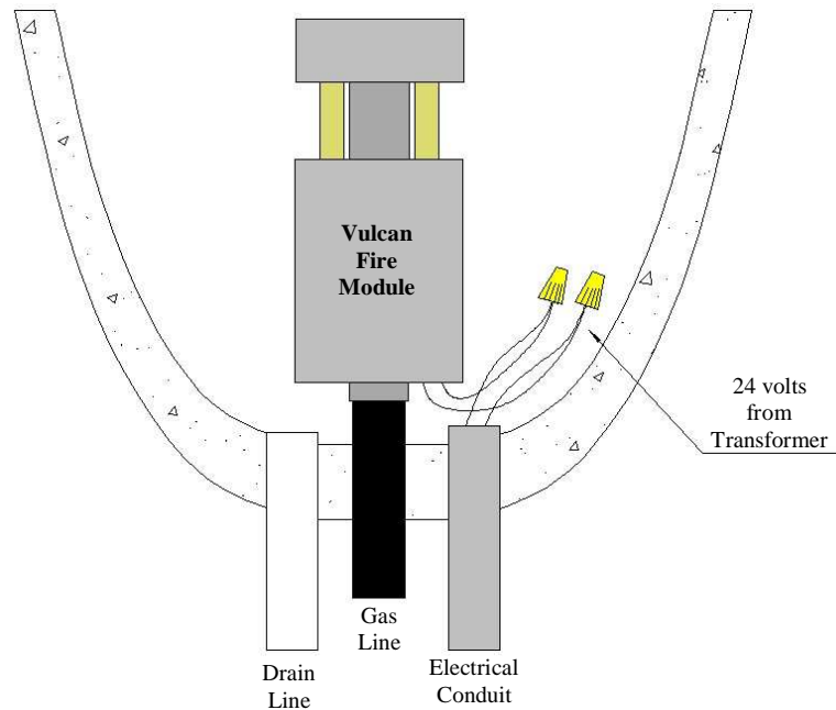
Illustration of Properly Installed Vulcan Fire Module (when complete)
