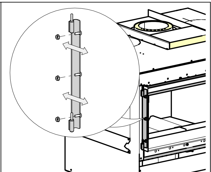
Figure 27 Door Hinge Adjustment
