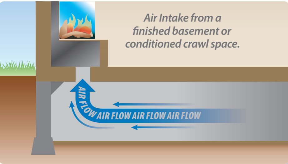
HIDDEN INTAKE CONSTRUCTION — URBANA EXCLUSIVE Where approved by local codes and the building's HVAC supplier, the chase intake air may be supplied from a basement or conditioned crawl space below if no visible open area is desired at the bottom of the chase.
