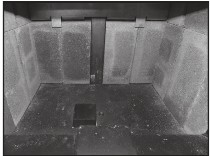
Figure 22: Firebox floor with ash dump.
