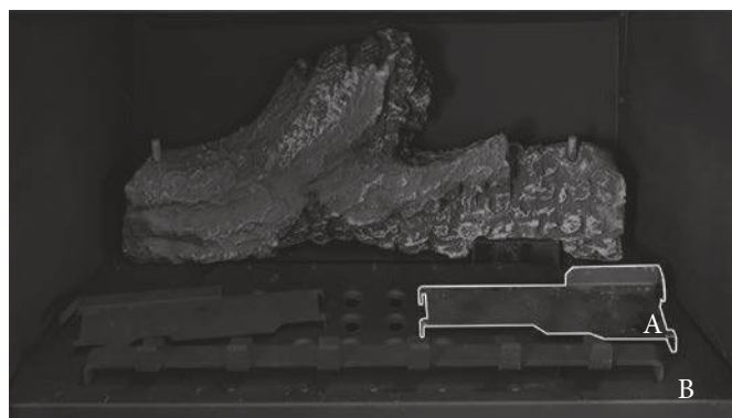
4. Locate notches on log stand (A) into holes on log deflector. (B)
