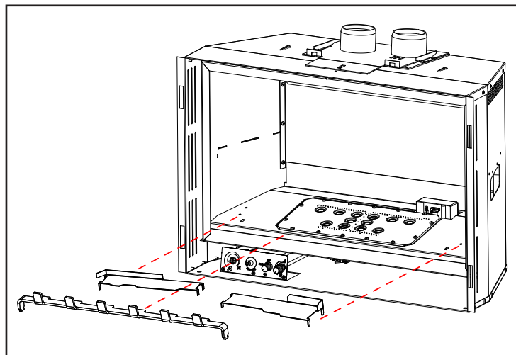
2. Remove log stands and log grate. Be careful not to scratch the paint when removing from fireplace.
