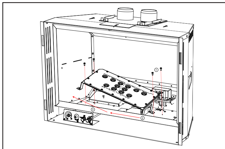
6. Unscrew the 4 fasteners holding down the burner and burner mount. Slide burner and mount to the left.
