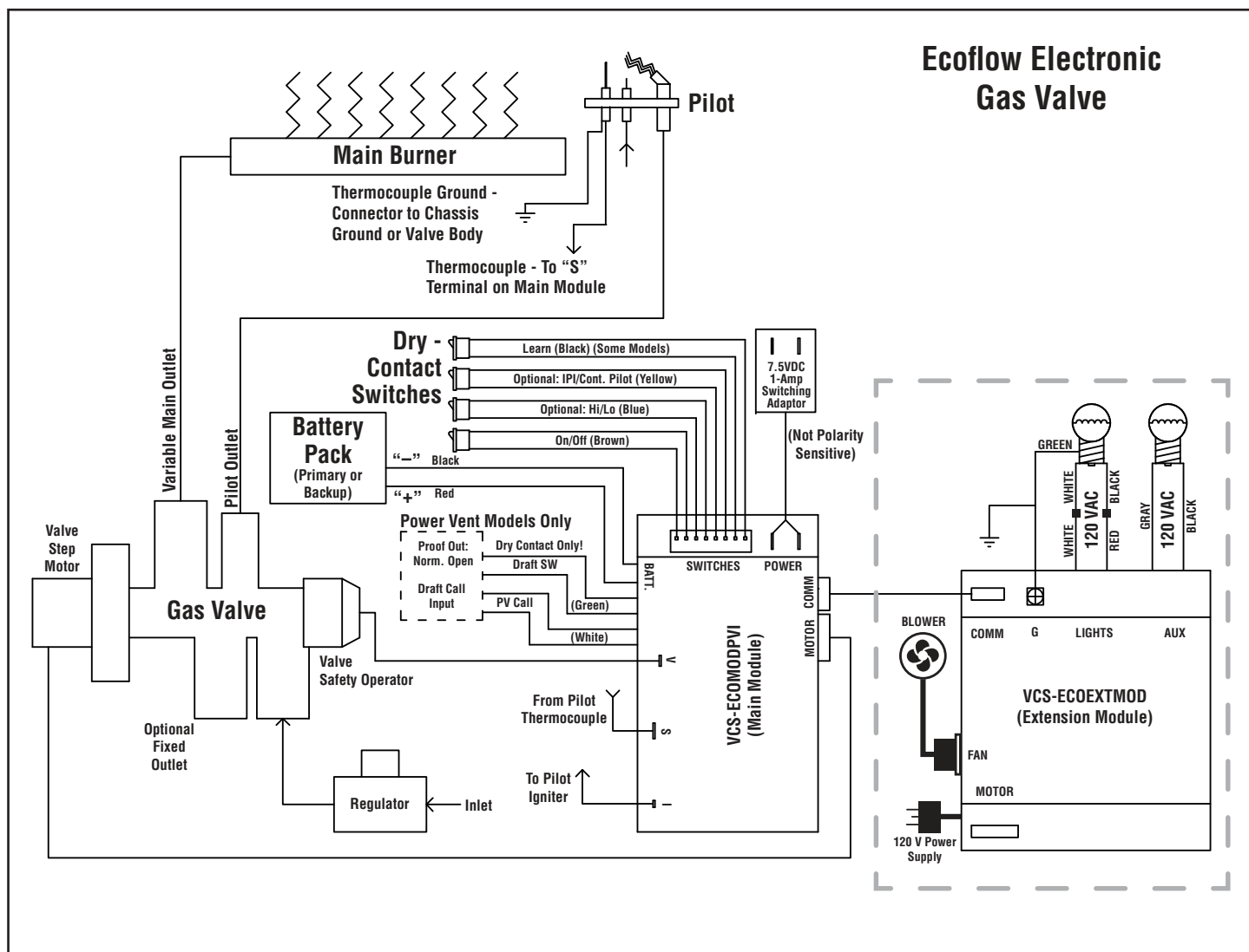
Figure 30A - Wiring Diagram—CompassDLX(35, 45, 55)TEN models
