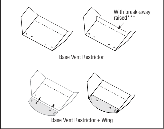
Figure 12 - Vent restrictor assembly
