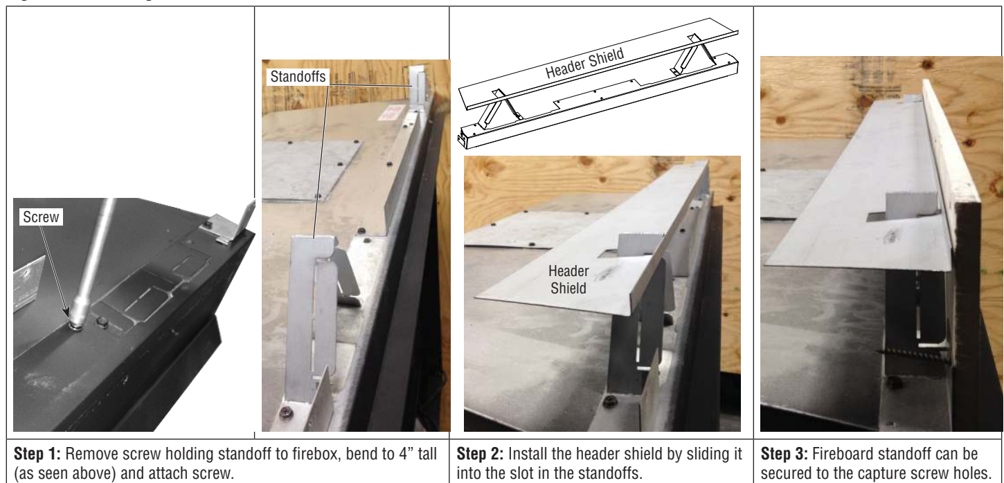
Figure 9 - Installing Header Shield
