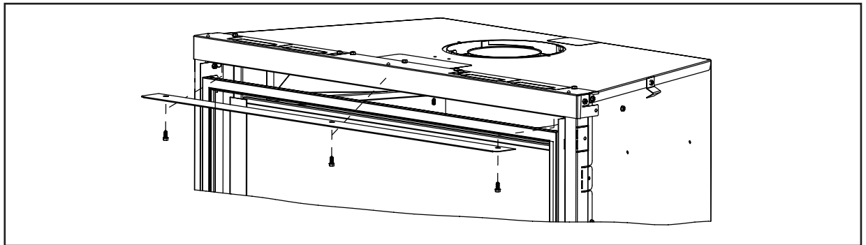
Figure 36 - Hood Installation
