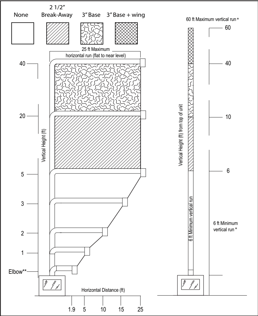
Figure 10 - When to use a vent restrictor
