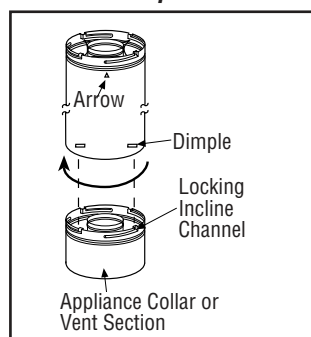
Figure 13 - Connecting vent components
