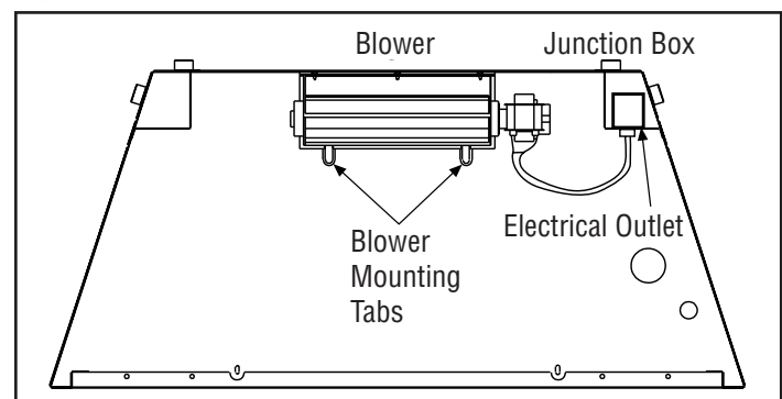
Figure 38 - Blower Installation
