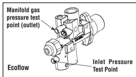
Figure 1 - MANIFOLD Outlet Gas Pressure Test Point
