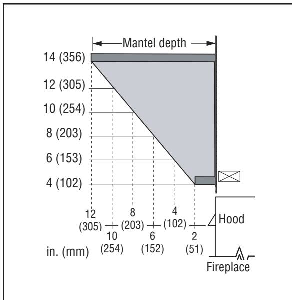
Figure 5 - Mantel Height Standard Compass Models
