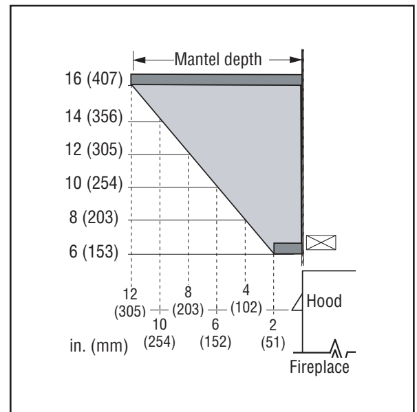
Figure 5A - Mantel Height Compass DLX Models
