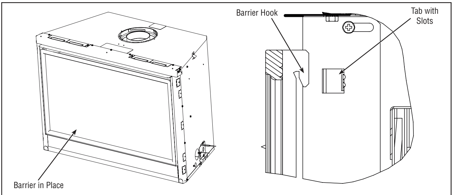
Figure 37 - Barrier Installation - Barrier Hook View
