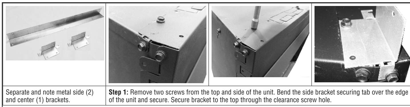
Figure 7B - Installing Non-Combustible Front Fireboard Standoff
