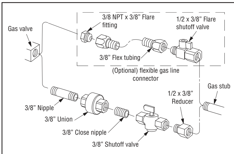
Figure 31 - Gas Line Connection
