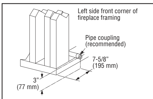
Figure 8 - Routing the gas line - all models
