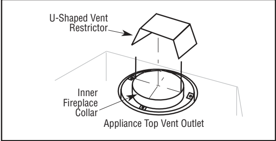
Figure 11 - Vent restrictor installation, Top vent
