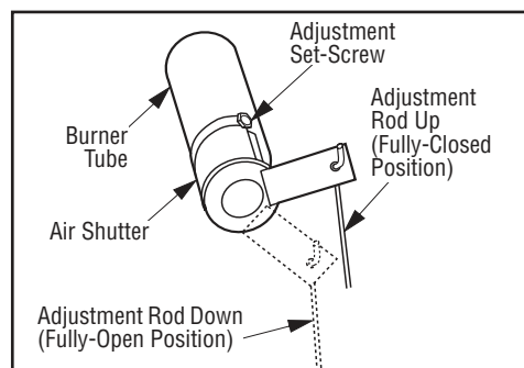
Figure 34 - Air Shutter Adjustment Rod
