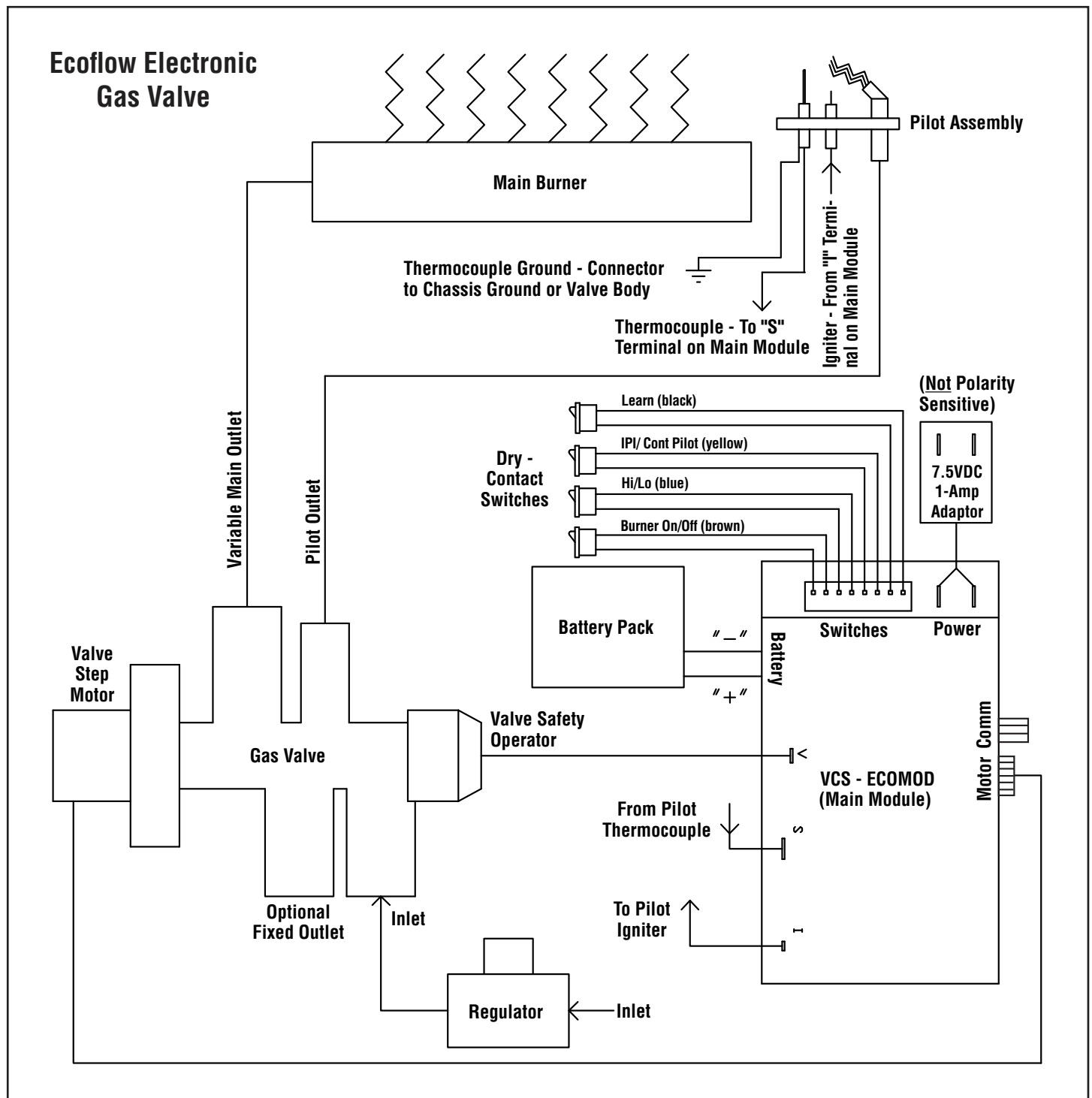
Figure 30 - Wiring Diagram—Compass(35, 45, 55)TEN models
