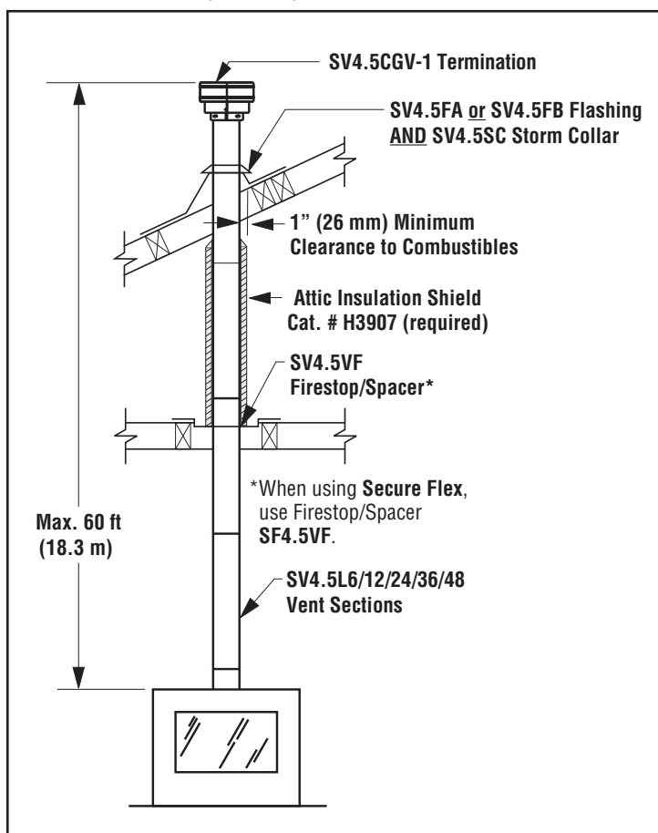
Figure 17 - Vertical (Straight) Installation
