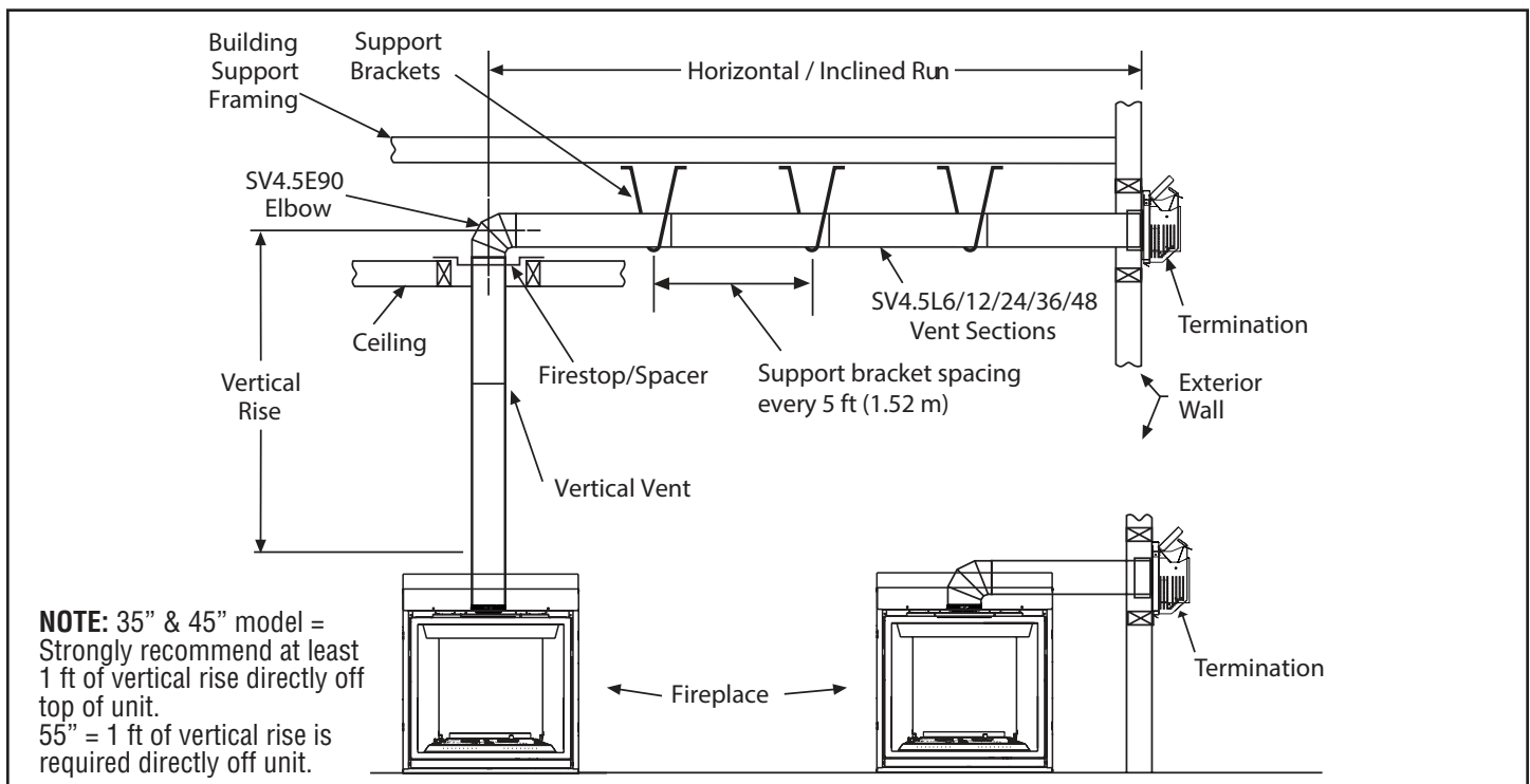
Figure 23 - Typical Horizontal Vent Installation
