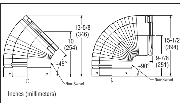
Figure 15 - Elbow Dimensions
