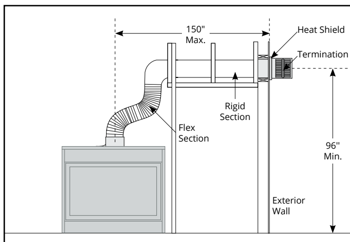
Figure 8.h Top Vented, wall mounted Multi-elbow installation. See Venting Graph for Top vent, wall mounted terminations
