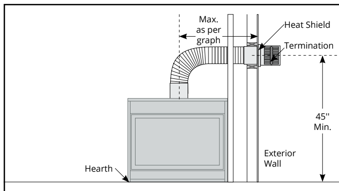
Figure 8.b Top Vented, wall mounted installation with 1 elbow (1 one 90° bend). The vent run must comply with Venting Graph for Top vent, wall mounted terminations
