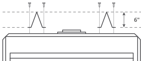
Figure 4.b Installing standoffs
