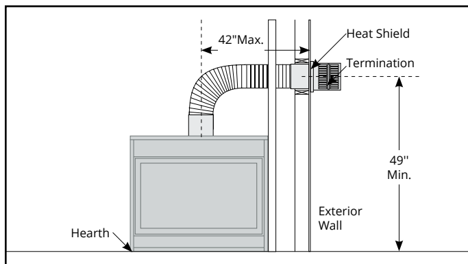
Figure 8.g Top Vented, wall mounted installation with 1 elbow (1 one 90° bend). The vent run must comply with Venting Graph for Top vent, wall mounted terminations
