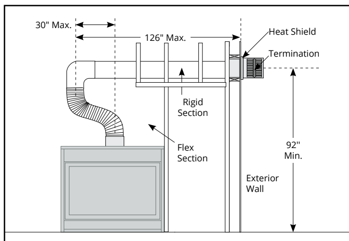
Figure 8.d Top Vented, wall mounted Retracted Multi-elbow installation
