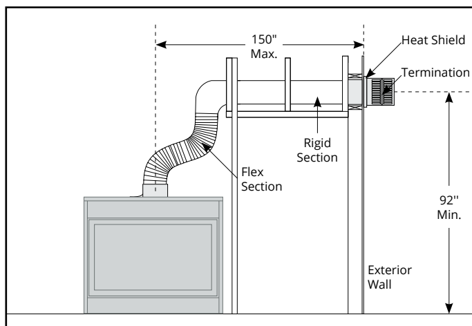
Figure 8.c Top Vented, wall mounted Multi-elbow installation. See Venting Graph for Top vent, wall mounted terminations
