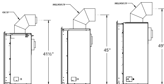
Figure 5.b Vent centers for top venting.
