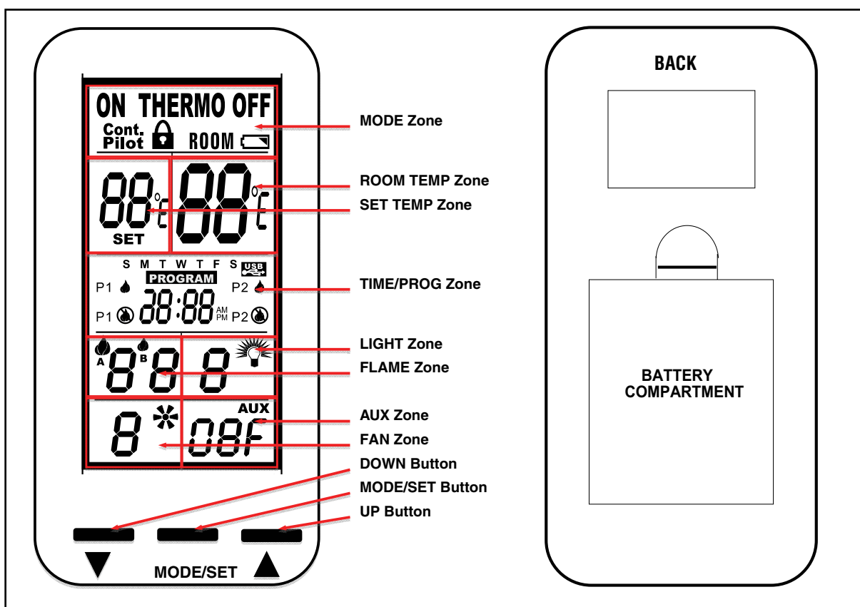
Figure 33 - Remote Control
