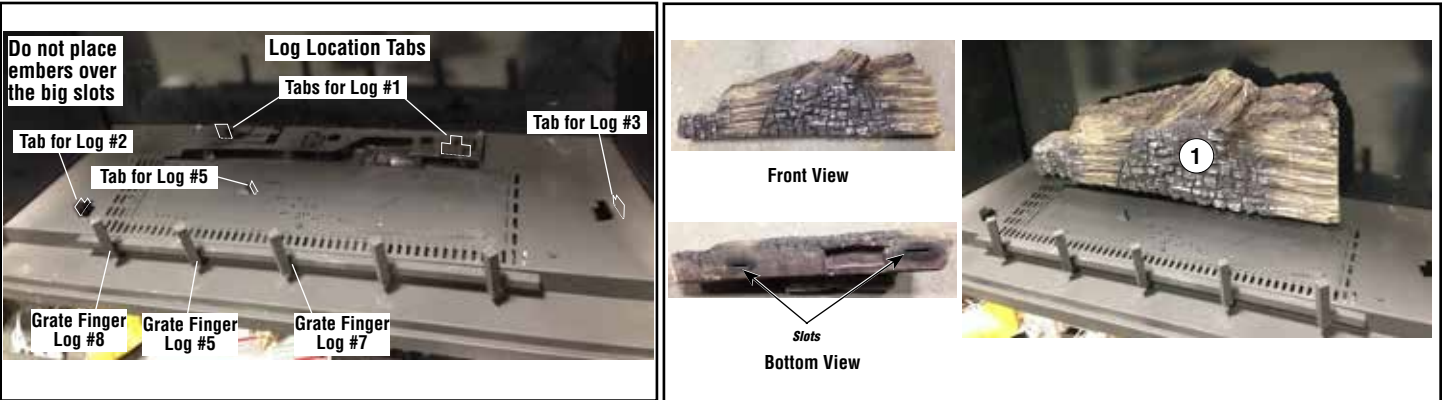
Figure 63 - Locate the log placement tabs
