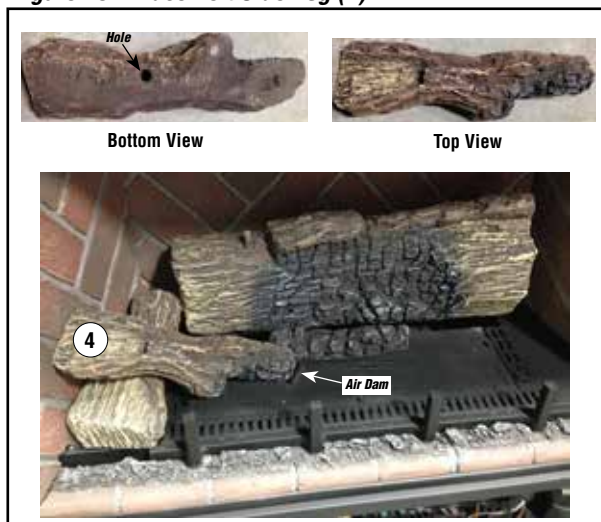
Figure 45 - Place Left Side Log (4)
