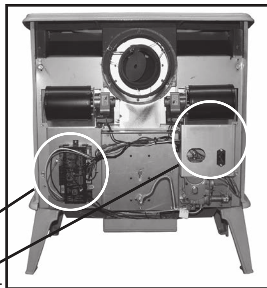
Figure 67: IFC module and ON - Off switch location.
