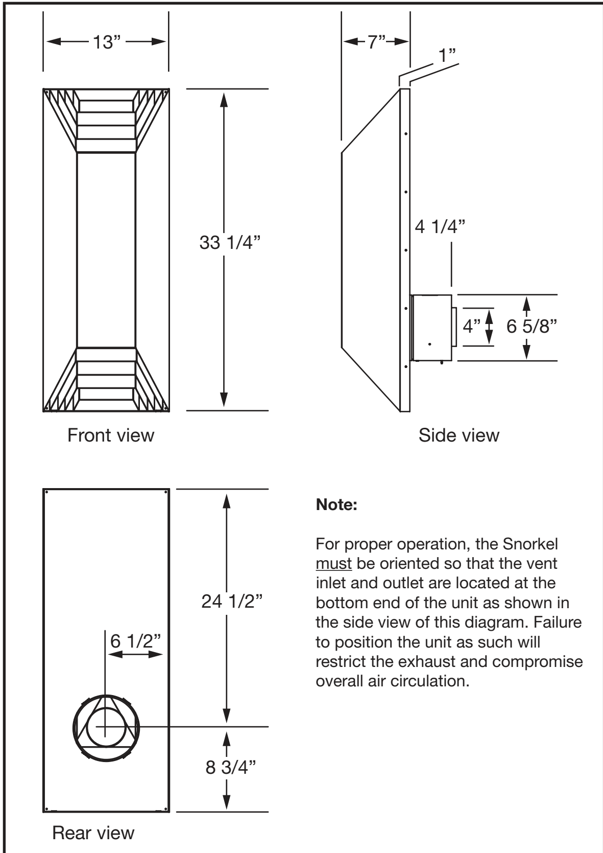
Figure 27: Snorkel dimensions.
