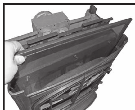
Figure 38: Trenton safety screen removal.
