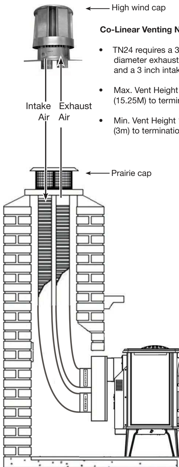
Figure 26: Trenton co-linear venting configuration.
