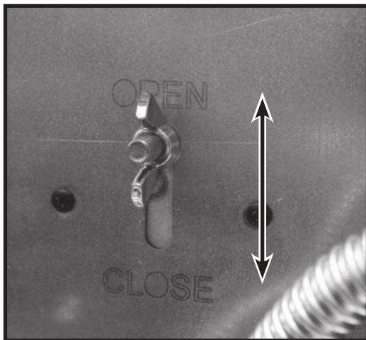
Figure 69: Venturi adjustment.
