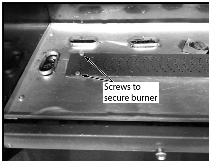
Figure 46: Burner.
