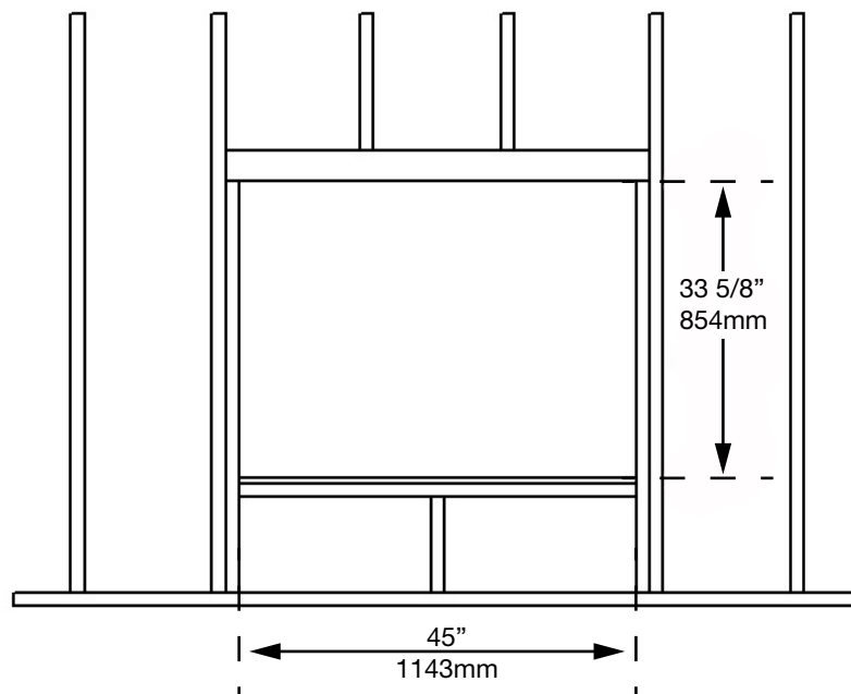
Figure 25: Framing dimensions.
