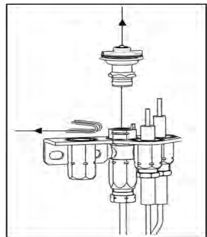
Figure 37: Pilot hood removal.
