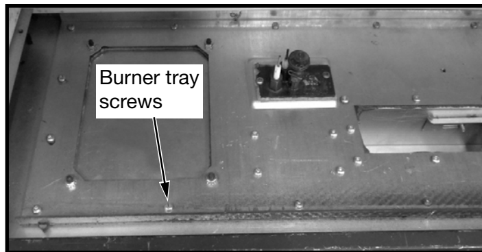
Figure 45: Burner tray.
