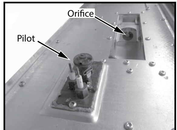
Figure 36: Orifice and pilot.
